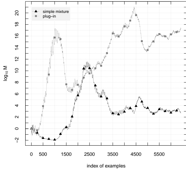
Figure 5: The growth of the simple mixture martingale and the plug-in martingale for the Statlog Satellite dataset. For the examples in the original order the exchangeability assumption is rejected: the final value of the simple mixture martingale is 5.6 \times 10^2 , and the final value of the plug-in martingale is 1.8 \times 10^{17} .
