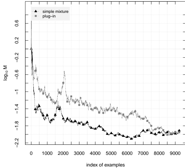
Figure 2: The growth of the simple mixture martingale and the plug-in martingale for the USPS dataset randomly shuffled before on-line testing. The exchangeability assumption is satisfied: the final values of the martingales are about 0.011.
