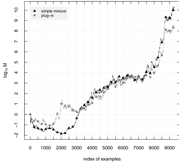
Figure 4: The growth of the simple mixture martingale and the plug-in martingale for the full USPS dataset. For the examples in the original order the exchangeability assumption is rejected: the final values of the martingales are greater than 3.8 \times 10^8 .
