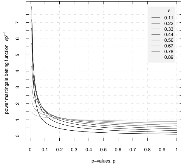
Figure 1: The betting functions that are used to construct the power and simple mixture martingales. The functions provide growth of the martingales for small p-values.
