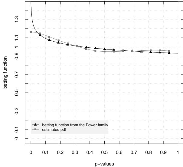
Figure 6: The “best” betting functions for testing the USPS dataset, the examples arriving in the original order. The best power function \varepsilon^* p^{\varepsilon^* - 1} is chosen according to the maximal final value of the power martingales. The betting function for the plug-in martingale is the estimated pdf.
