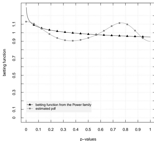
Figure 7: The “best” betting functions for testing the Statlog Satellite dataset, the examples arriving in the original order. The best power function \varepsilon^* p^{\varepsilon^* - 1} is chosen according to the maximal final value of the power martingales. The betting function for the plug-in martingale is the estimated pdf.
