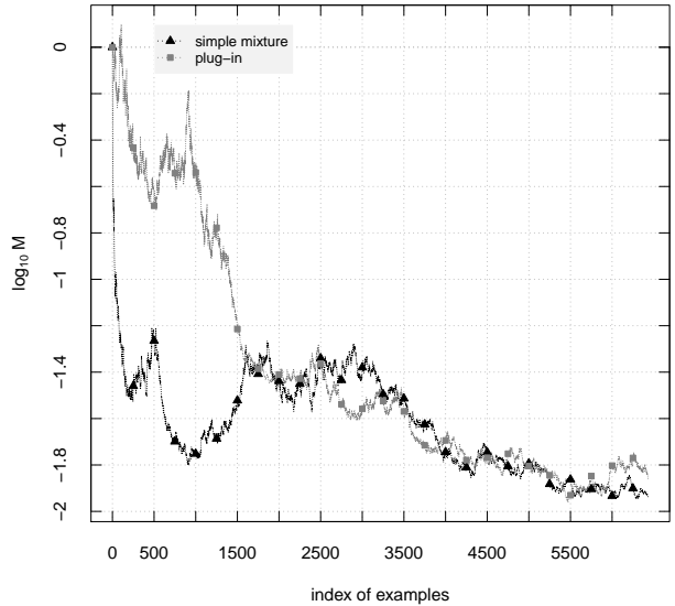
Figure 3: The growth of the simple mixture martingale and the plug-in martingale for the Statlog Satellite dataset randomly shuffled before on-line testing. The exchangeability assumption is satisfied: the final values of the martingales are about 0.01.
